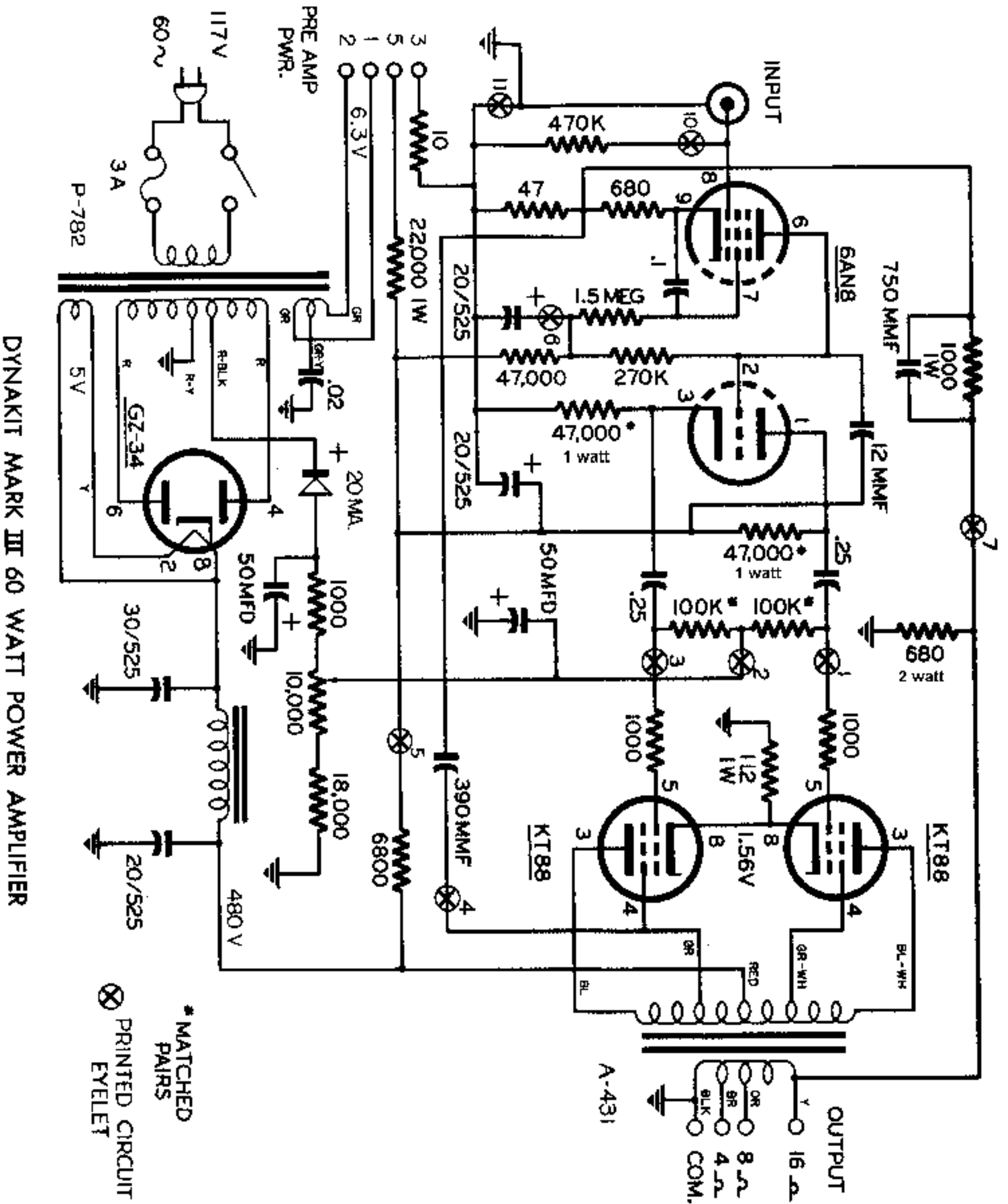
"Classic" Dynaco Circuit
